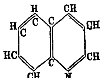
Quinoline.
